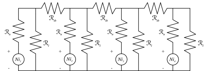
Fig. 3. Magnetic circuit model for four-phase coupled inductor. From [1].
