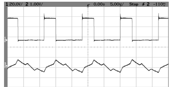
Fig. 6. Waveforms with poor coupling. The upper waveform shows the rectangular waveform produced by the switch (20 V/div). The lower waveform shows the ac component of inductor current (10 A/div). The time scale is 5 \mu s/div.
