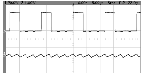
Fig. 5. Waveforms with good coupling. The upper waveform shows the rectangular waveform produced by the switch (20 V/div). The lower waveform shows the ac component of inductor current (10 A/div). The time scale is 5 \mu s/div.
